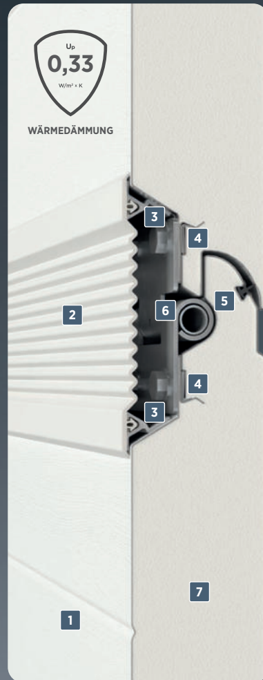
Tor: MakroTherm 2.0, MakroTherm XXL (1)
